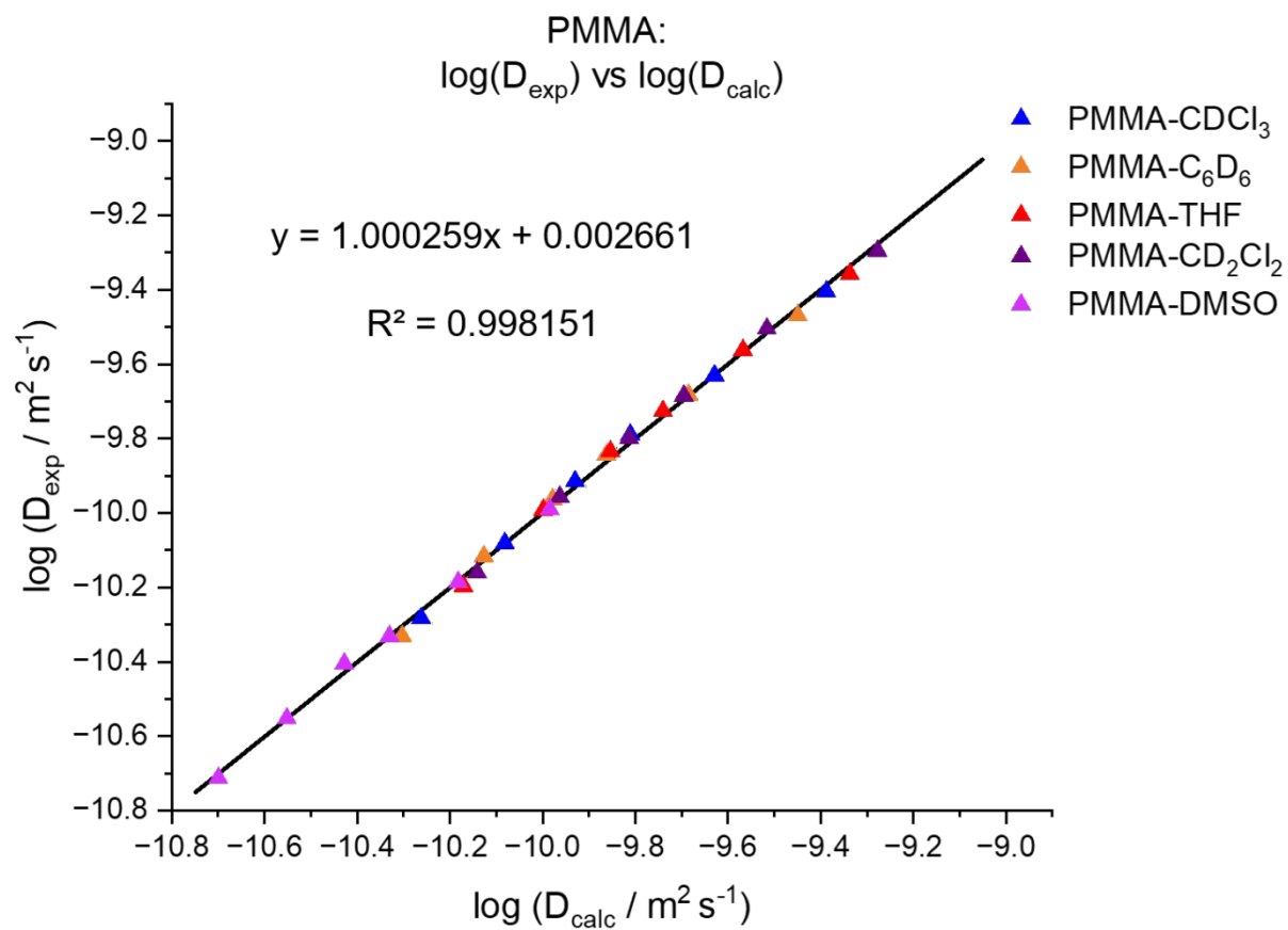
Figure S14: Experimental diffusion coefficients vs. calculated diffusion coefficients via equation (13) for PMMA.
